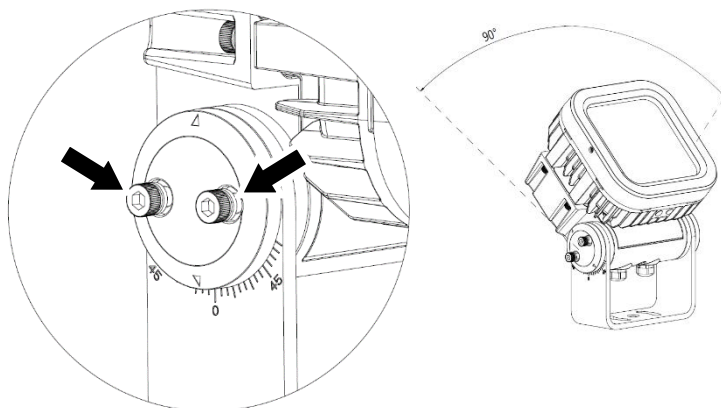
Figure 3. Tilt adjustment
