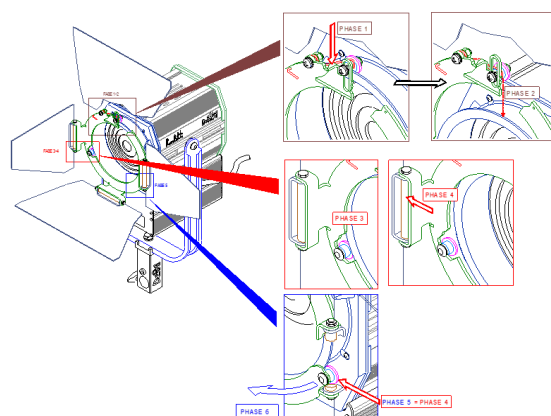
BARNDOOR DISASSEMBLING
