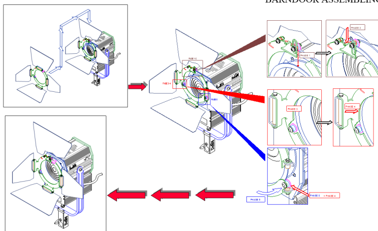
BARNDOOR ASSEMBLING
